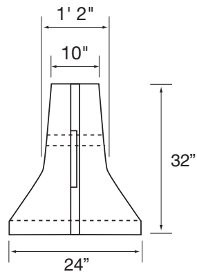
END VIEW
