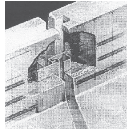
J-J Hook Cut-Away
